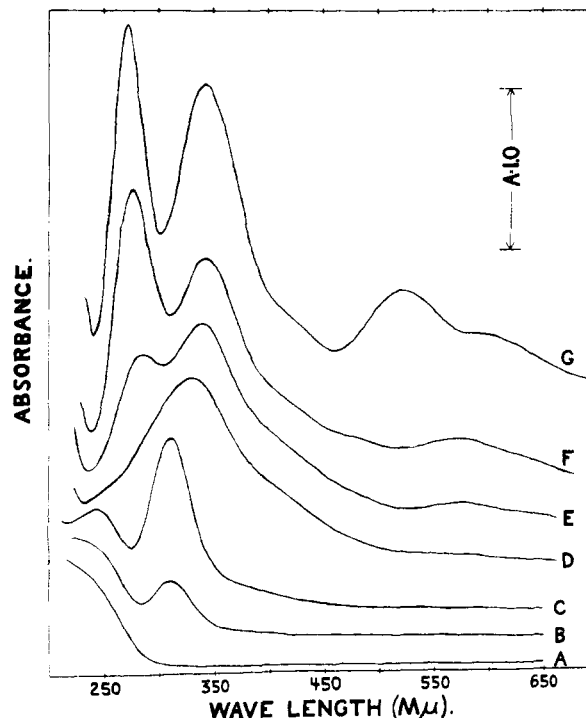
Fig. 1.—Cu(ClO 4 ) 2 concentration in ethanol was 4.00 × 10 -3 M; varying amounts of LiBr were added: A, no LiBr; B, 1.00 × 10 -3 M; C, 4.00 × 10 -3 M; D, 25.0 × 10 -3 M; E, 75.0 × 10 -3 M; F, 720 × 10 -3 M; G, 2800 × 10 -3 M (path length, 0.1 cm.).
